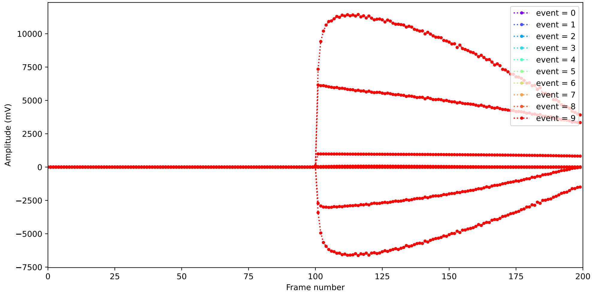
Pixel signals, all pixels from event 0 to 9
